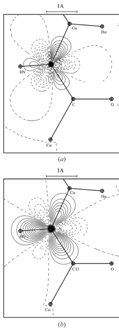
Figure 1 Deformation electron density of the N atom ( a ) using the KVC parameters and ( b ) calculated with the P2JL parameters. Contours are at 0.05 \text{ e } \text{Å}^{-3} with full lines denoting positive contours and dashed lines denoting negative and zero contours.
