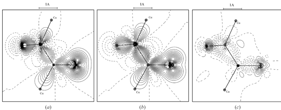
Figure 2 Static deformation electron densities of the \text{NH}-\text{C}'=\text{O} group, ( a ) using the KVC parameters, ( b ) calculated with the P2JL parameters, and ( c ) the difference between ( a ) and ( b ). Contours are as in Fig. 1.
